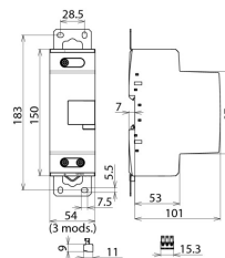
Dimensions DBM 1 CI 760 FM
