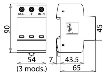
Dimensions DG YPV SCI 1000
