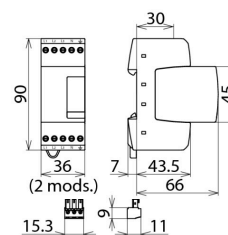
Dimensions DR M 4P 255 FM
