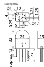
Dimensions VC 280 2
