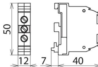
Dimensions SLK 16
