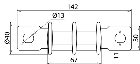
Dimensions DSFS
