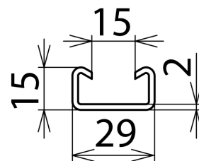
Dimensions AS SAK 1000 V2A
