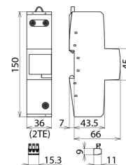
Dimensions DGPM 1 255 FM
