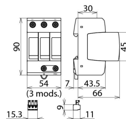
Dimensions DG M TNC 150 FM
