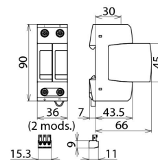
Dimensions DG M TN 150 FM
