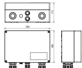
Dimensions DCU 2 YPV 1100 2M 1S
