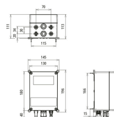
Dimensions DCU 1+2 YPV 2M 1S MC4
