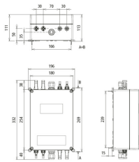
Dimensions DCU S 2 YPV 1+2 1200 2M 1S MC4
