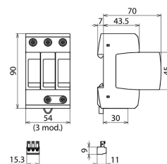
Dimensions DG MP TNC ACI 275 FM
