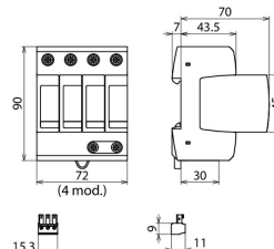
Dimensions DG M TNS ACI 275 FM
