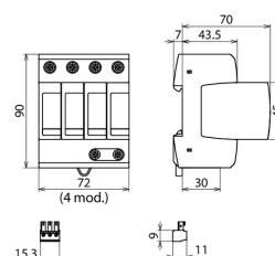
Dimensions DG M TT ACI 275 FM
