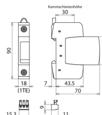
Dimensions DG S ACI 385 FM
