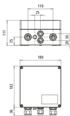
Dimensioni DCU 2 YPV 1+2 1000 1M 2S FM
